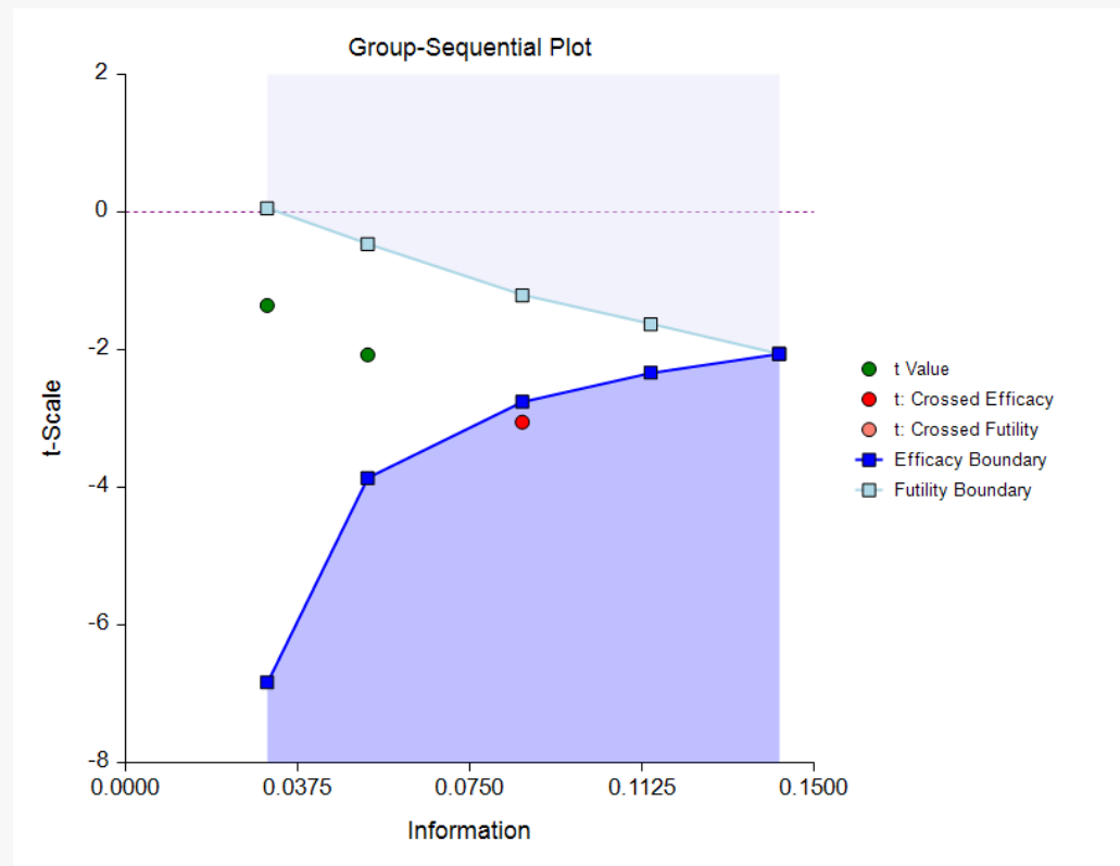
Group-Sequential Boundary Plot at Stage 3
