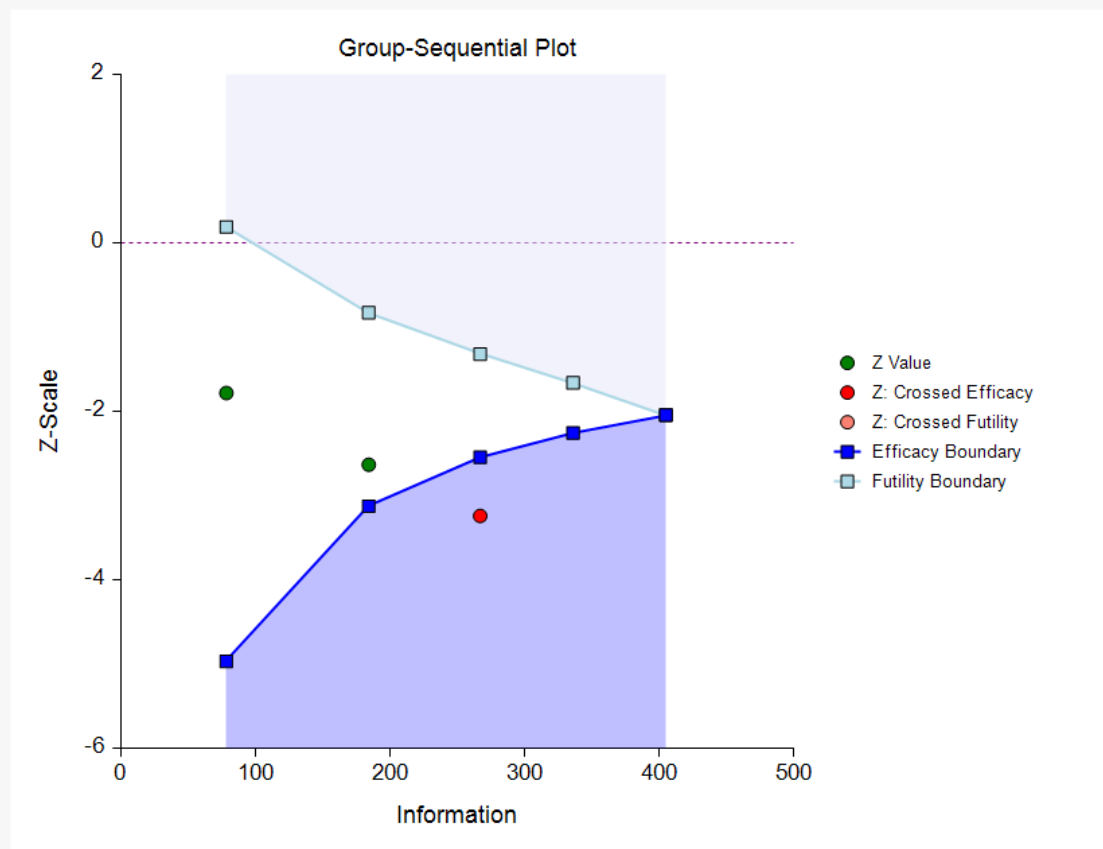
Group-Sequential Boundary Plot at Stage 3
